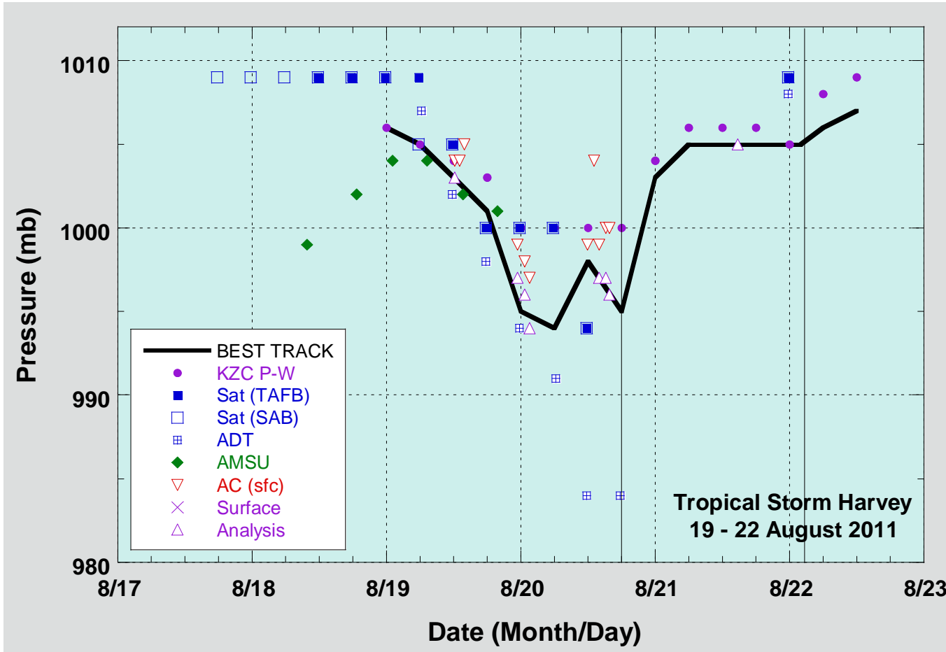
Figure 3. Selected pressure observations and best track minimum central pressure curve for Harvey. Advanced Dvorak Technique (ADT) estimates courtesy of UW-CIMSS. Dashed vertical lines correspond to 0000 UTC. Solid vertical lines represent when the cyclone made landfall. KZC P-W refers to pressure estimates derived by applying the Knaff-Zehr-Courtney pressure-wind relationship to the best track wind speeds. AMSU estimates are derived from the UW-CIMSS technique.
